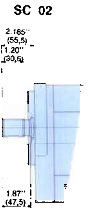
Splined shaft
