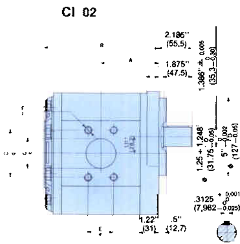
Parallel Shaft
